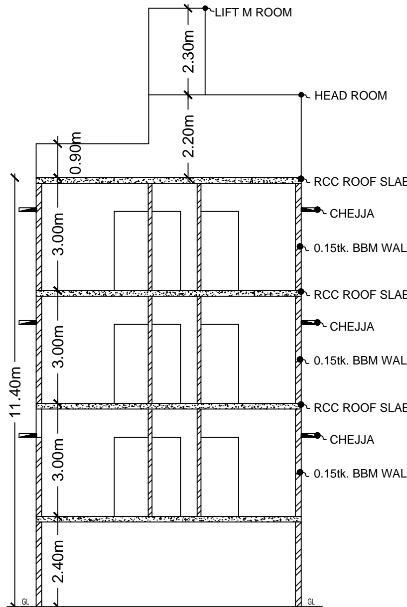
SECTION @ X-X'
