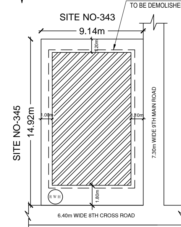
SITE PLAN
